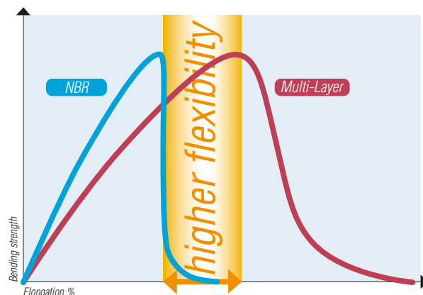
Elastic properties
